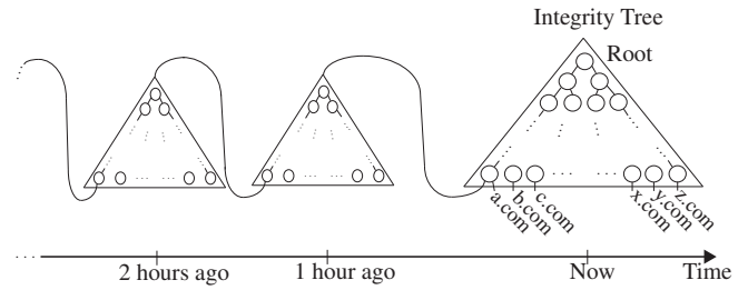
Figure 2: AKI Integrity Tree structure.
